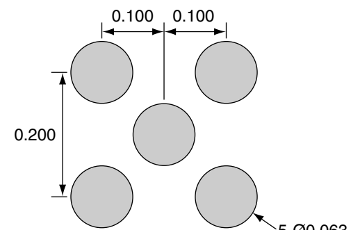
RECOMMENDED FOOTPRINT
